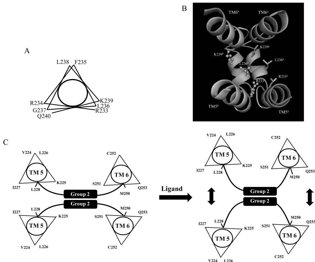
Figure 8. Helical wheel projections and 3D model of IL3 residues involved in Ste2p–Ste2p interactions. (A) The IL3 residues R233 to Q240 are suggested to form a 3_{10} helix structure with a periodicity of 3.2 residues per turn in the helical wheel. 58 (B) The 3D structure of two Ste2p molecules showing regions TMS, TM6, and IL3 with a 3_{10} helix in IL3 as predicted by the Pyre Structural Bioinformatics Group prediction tools. 30 The IL3 3_{10} helices of two Ste2p subunits are suggested to be in close proximity that permit disulfide cross-linking. (C) A schematic diagram showing possible shifts at the cytoplasmic ends of TMS and TM6 upon ligand binding. The vertical arrows indicate a shift of the TMS away from each other.
